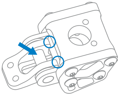
Shifter unit bottom view
